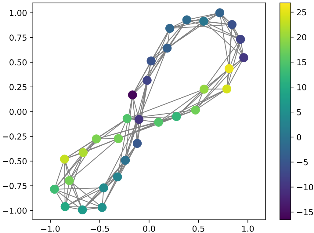
Generalized Laplacian of signal
