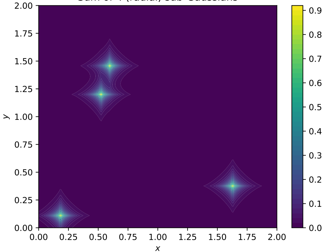
Sum of 4 (radial) sub-Gaussians
