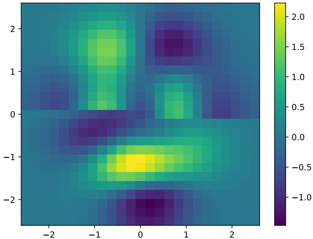
Directional derivatives in 1st direction
