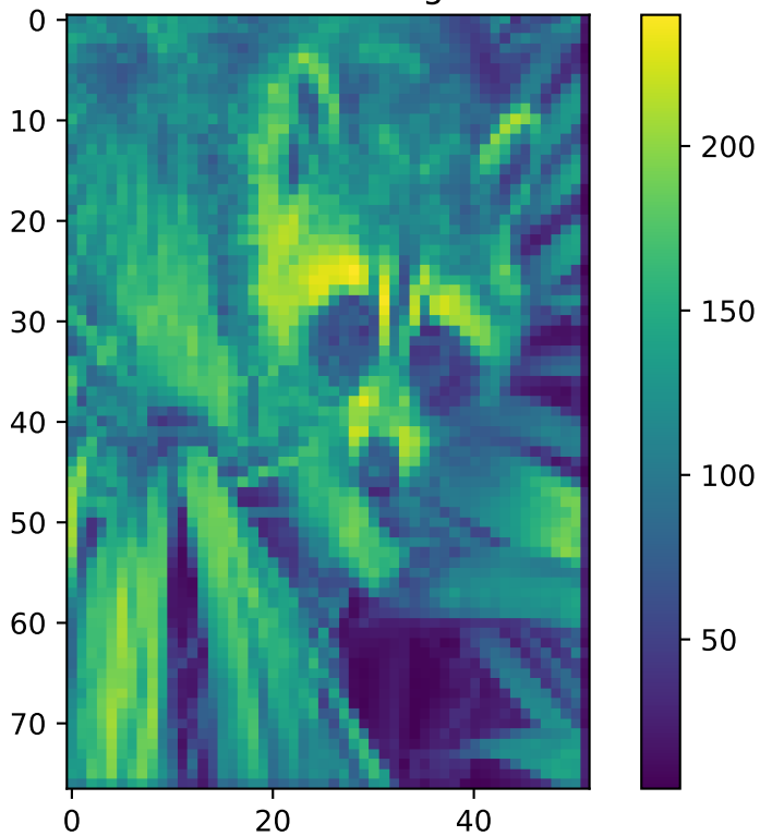
Mean Pooling
