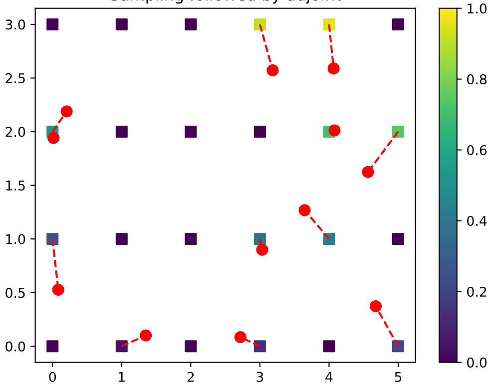
Sampling followed by adjoint
