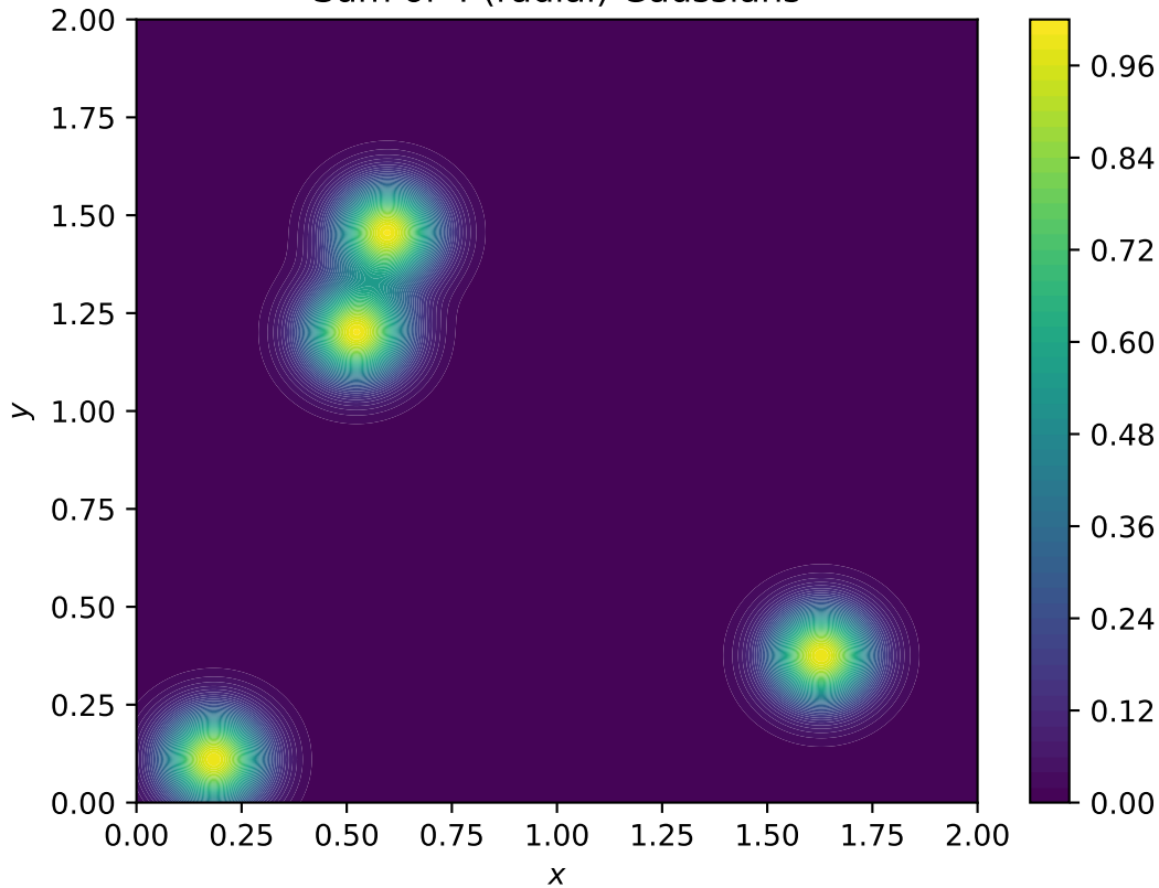
Sum of 4 (radial) Gaussians
