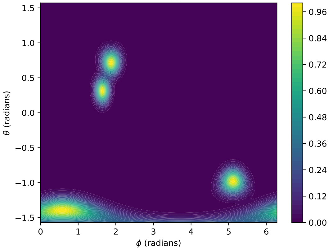
Sum of 4 (zonal) wrapped Gaussians
